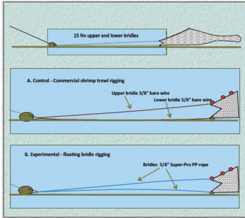
Figure 32. Floating bridles.
