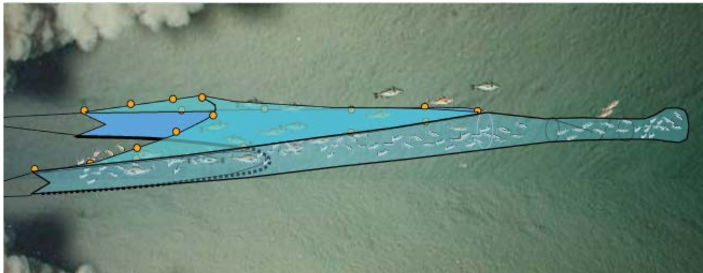
Figure 33. Topless shrimp trawl.
