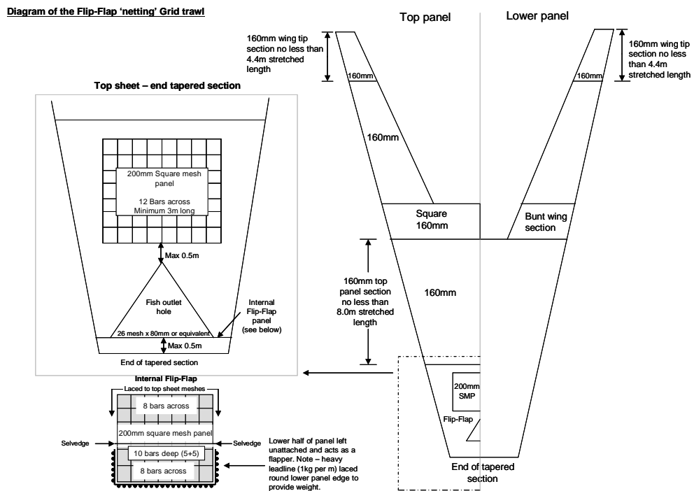
Figure 23. Scottish Flip/flap gear.
